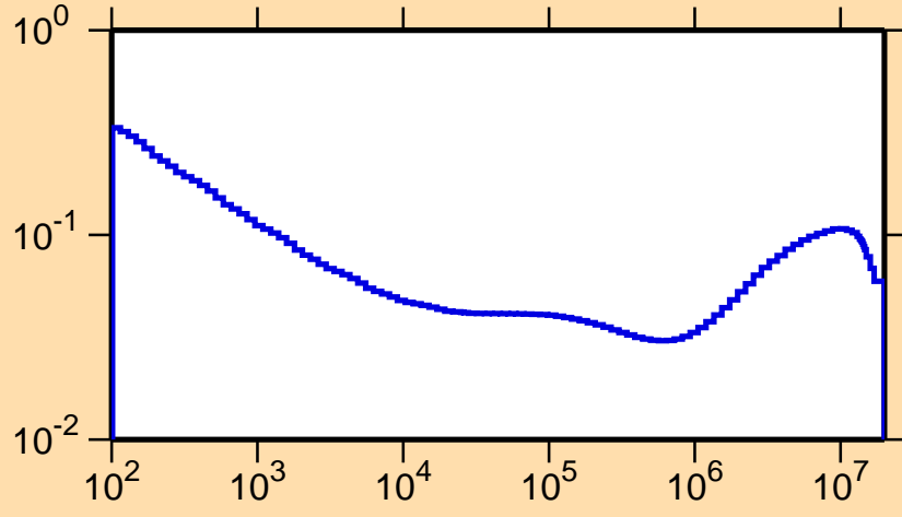
\sigma vs. E for ^{104}\text{In}(n,\alpha)
