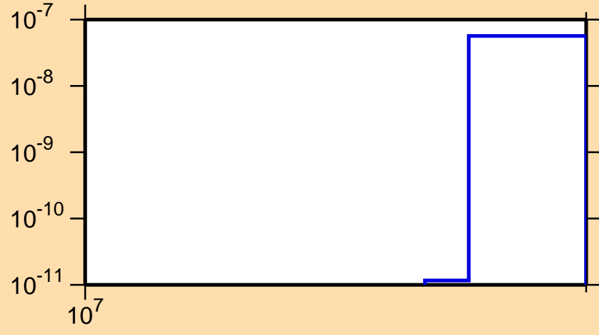
\sigma vs. E for ^{105}\text{In}(n,\text{pt})
