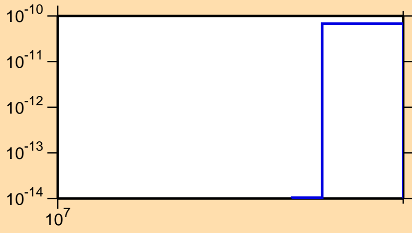
\sigma vs. E for ^{105}\text{In}(\text{mt } 34)
