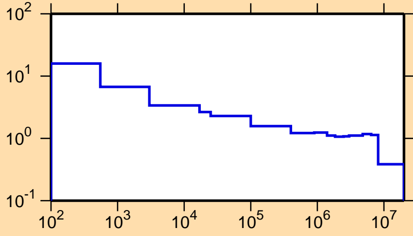
\sigma vs. E for ^{105}\text{In}(n,p)
