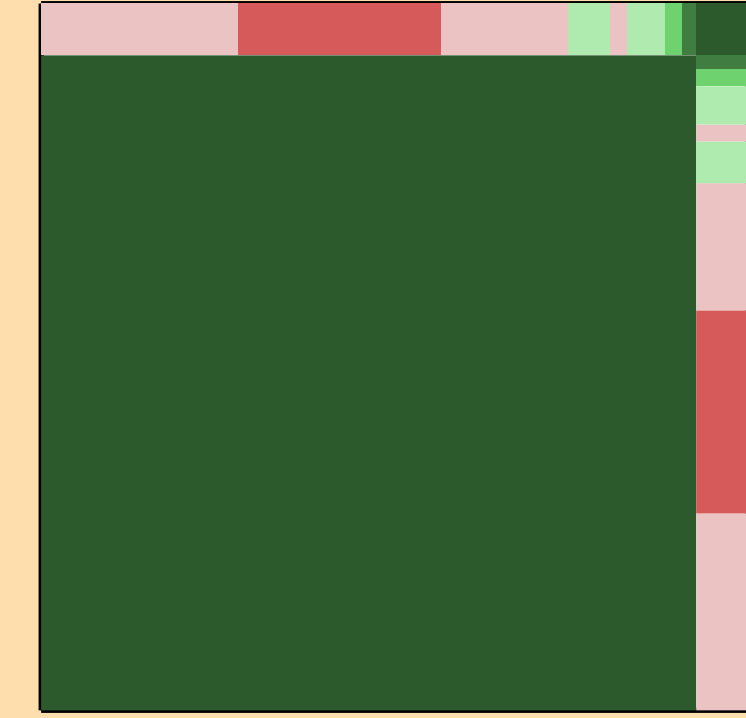
Correlation Matrix
