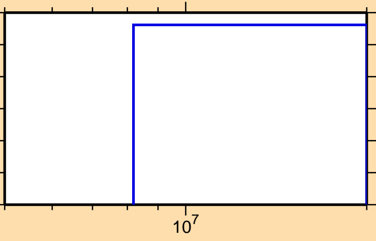
\sigma vs. E for ^{105}\text{In}(\text{mt } 45)
