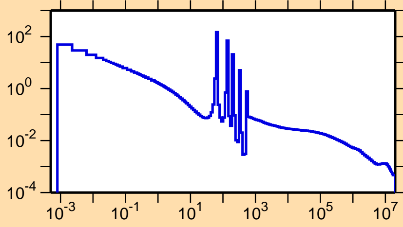
\sigma vs. E for ^{105}\text{In}(n,\gamma)
