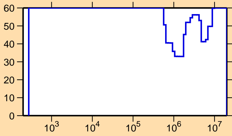
\Delta\sigma/\sigma vs. E for ^{105}\text{In}(n,p)
