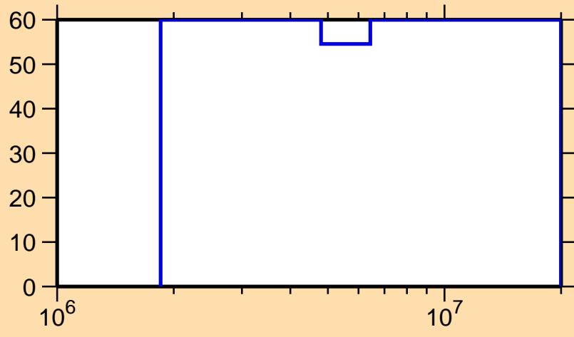
\Delta\sigma/\sigma vs. E for ^{105}\text{In}(n,n\text{cont.})
