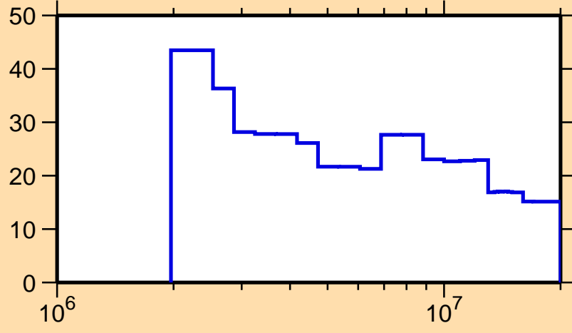
\Delta\sigma/\sigma vs. E for ^{106}\text{In}(n,n\text{cont.})
