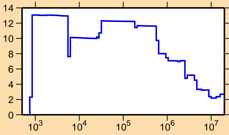
\Delta\sigma/\sigma vs. E for ^{106}\text{In}(n,\text{nonel.})
