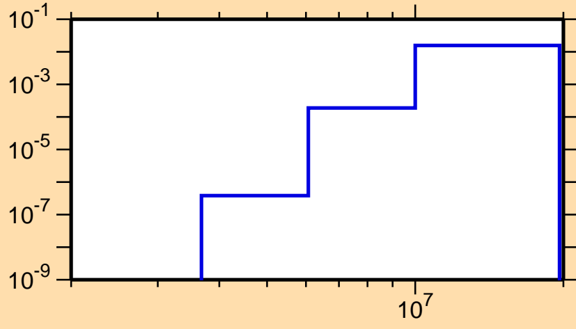
\sigma vs. E for ^{106}\text{In}(n,d)
