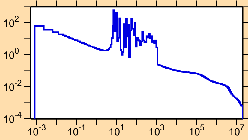
\sigma vs. E for ^{106}\text{In}(n,\gamma)
