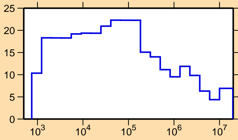
\Delta\sigma/\sigma vs. E for ^{106}\text{In}(n,el.)
