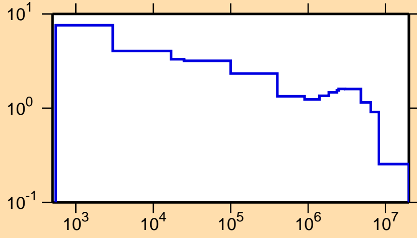
\sigma vs. E for ^{106}\text{In}(n,p)
