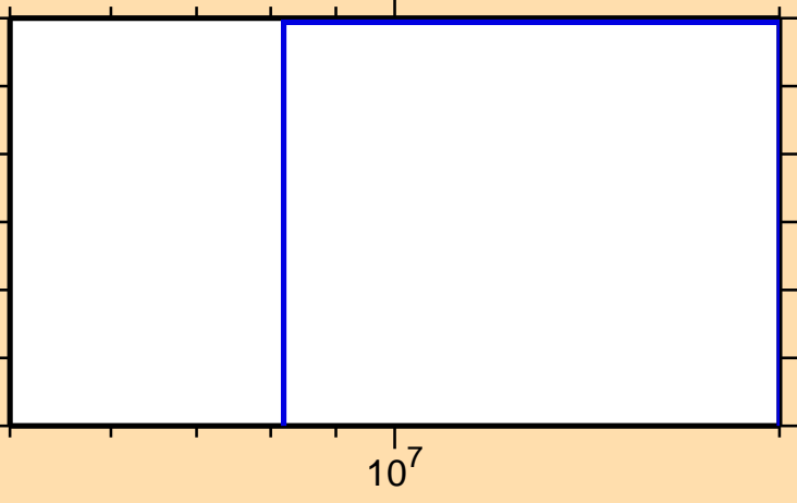
\sigma vs. E for ^{106}\text{In}(n,2n\alpha)
