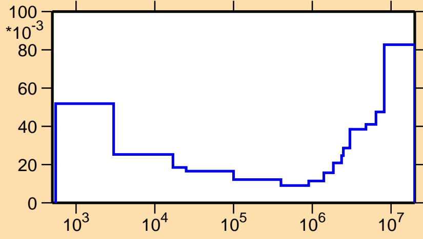
\sigma vs. E for ^{106}\text{In}(\alpha)
