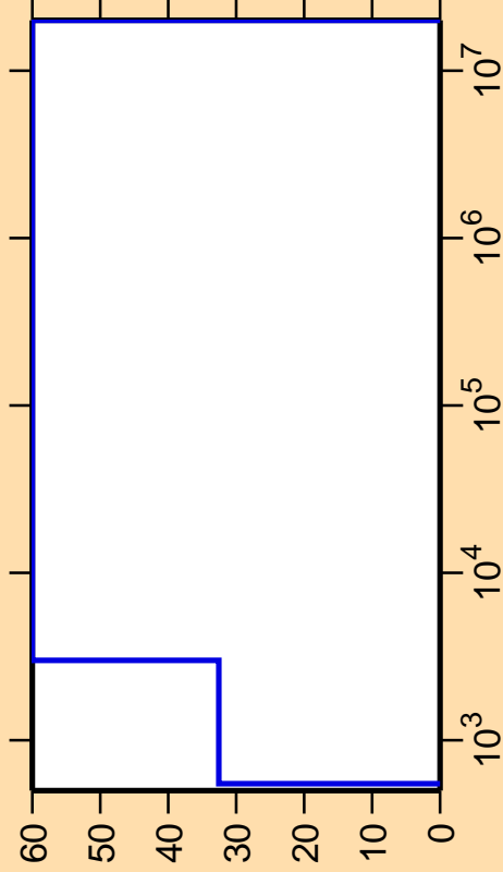
\Delta\sigma/\sigma vs. E for ^{106}\text{In}(\alpha)
