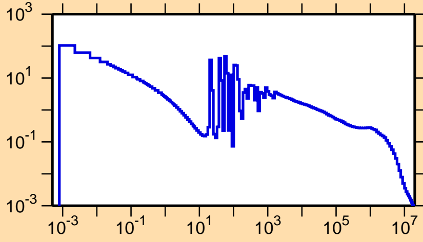
\sigma vs. E for ^{107}\text{In}(n,\gamma)
