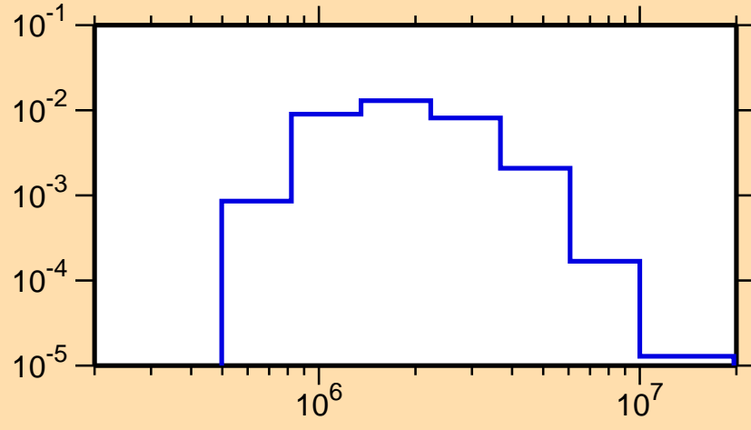
\sigma vs. E for ^{107}\text{In}(n,n_1)
