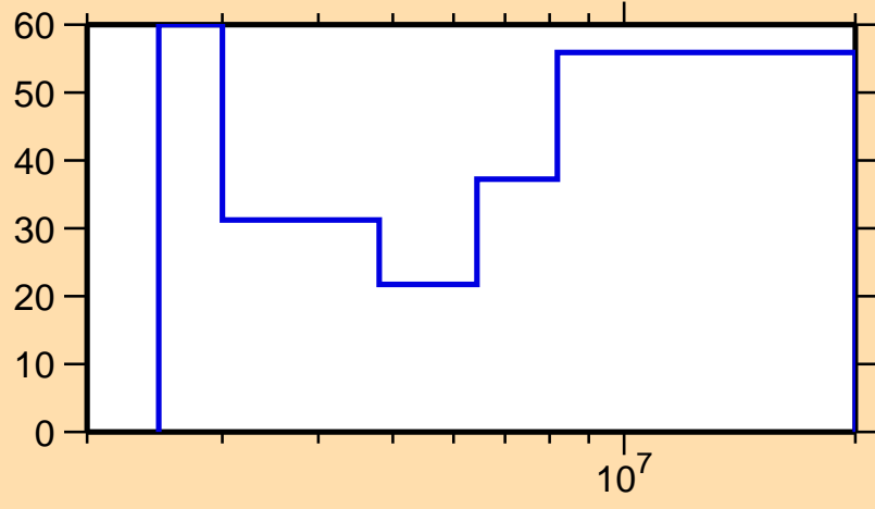
\Delta\sigma/\sigma vs. E for ^{107}\text{In}(n,n\text{cont.})
