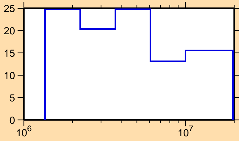
\Delta\sigma/\sigma vs. E for ^{107}\text{In}(n, el.)
