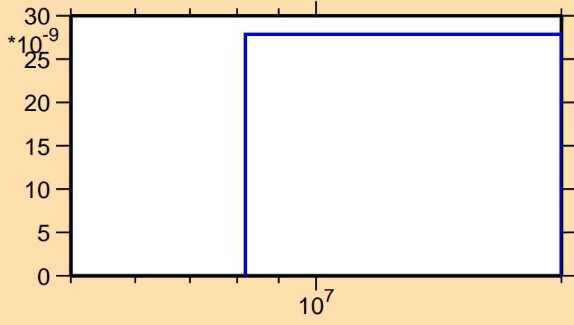
\sigma vs. E for ^{107}\text{In}(n,2n\alpha)
