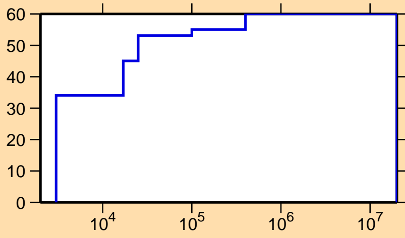
\Delta\sigma/\sigma vs. E for ^{107}\text{In}(n,p)
