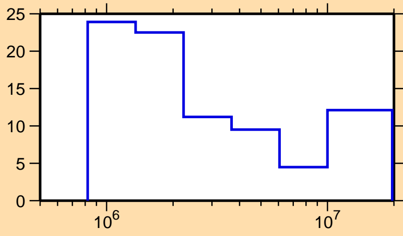
\Delta\sigma/\sigma vs. E for ^{108}\text{In}(n,\text{tot.})
