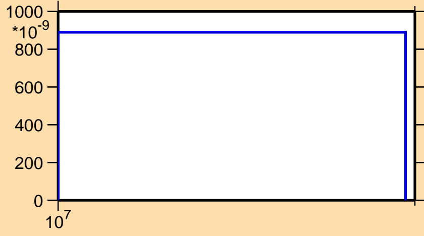
\sigma vs. E for ^{108}\text{In}(n,2n\alpha)
