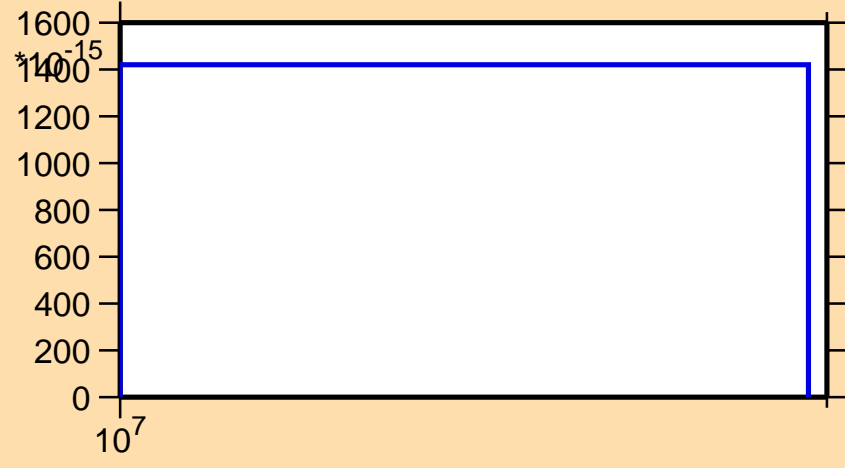
\sigma vs. E for ^{108}\text{In}(\text{mt } 34)
