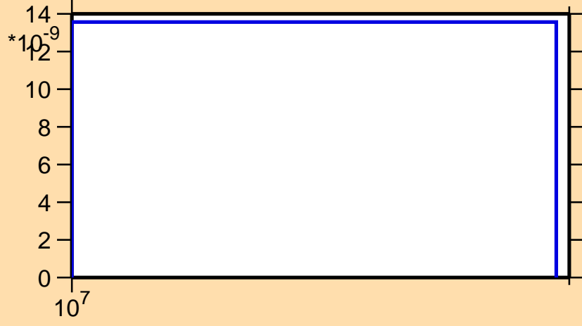
\sigma vs. E for ^{108}\text{In}(\text{mt } 45)
