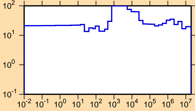
\Delta\sigma/\sigma vs. E for ^{108}\text{In}(n,\text{el.})
