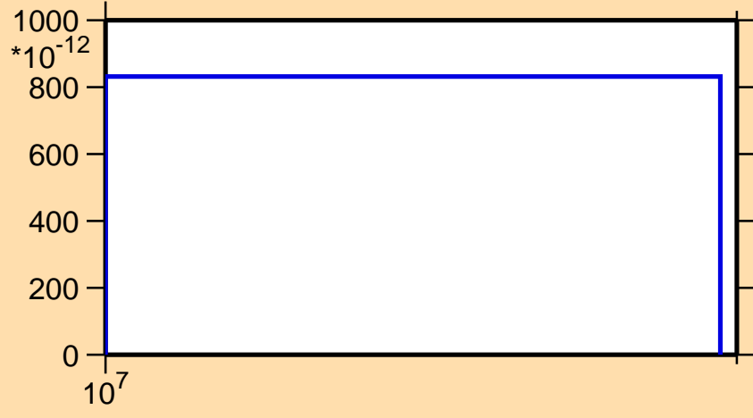
\sigma vs. E for ^{108}\text{In}(n,pd)
