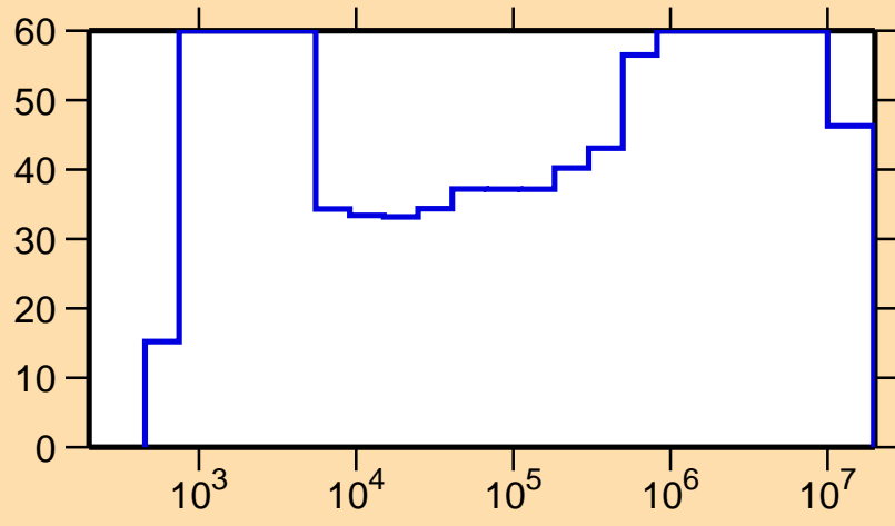
\Delta\sigma/\sigma vs. E for ^{108}\text{In}(n,p)
