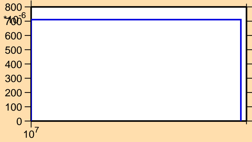
\sigma vs. E for ^{108}\text{In}(n,2np)
