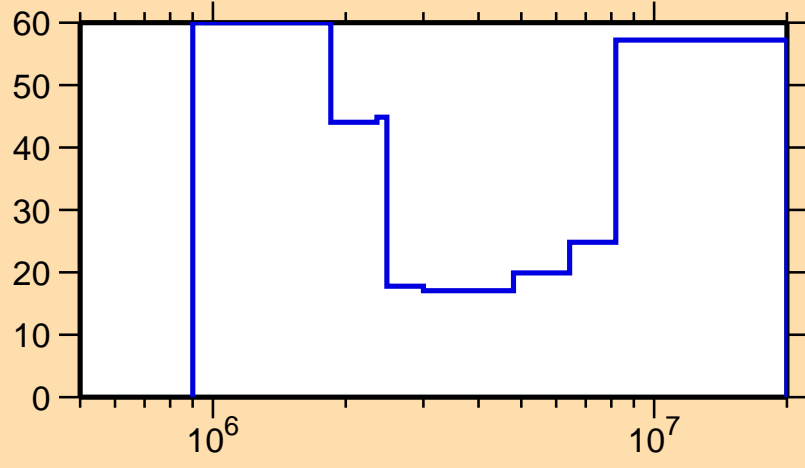
\Delta\sigma/\sigma vs. E for ^{108}\text{In}(n,n\text{cont.})
