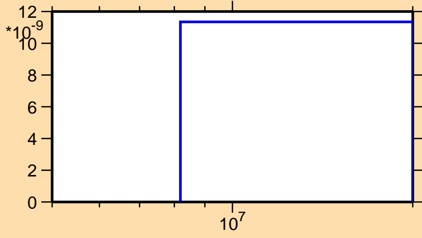
\sigma vs. E for ^{108}\text{In}(\text{mt } 45)
