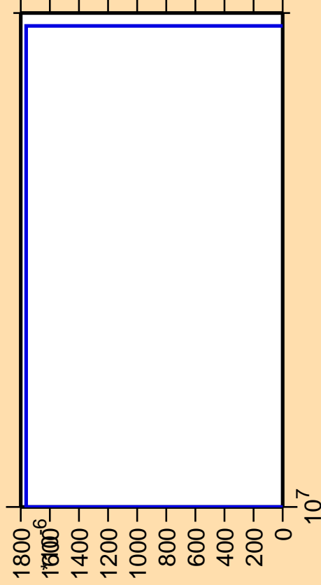
\Delta\sigma/\sigma vs. E for ^{109}\text{In}(n,\text{pt})
