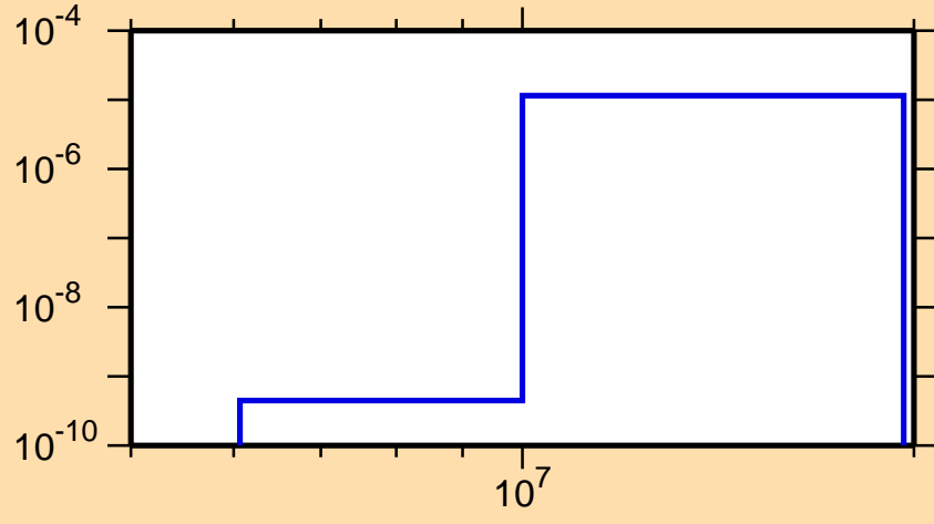
\sigma vs. E for ^{109}\text{In}(n,p\alpha)
