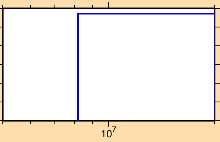
\sigma vs. E for ^{109}\text{In}(n,3n)
