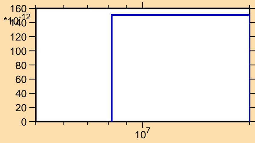
\sigma vs. E for ^{109}\text{In}(n,nt)
