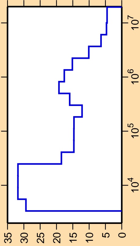
\Delta\sigma/\sigma vs. E for ^{109}\text{In}(n,\text{nonel.})
