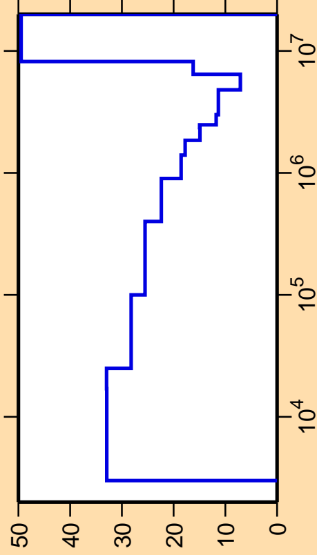
\Delta\sigma/\sigma vs. E for ^{109}\text{In}(n,\text{inel.})
