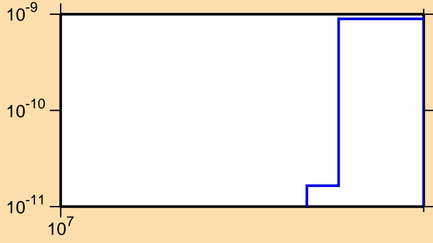
\sigma vs. E for ^{110}\text{In} (mt 45)
