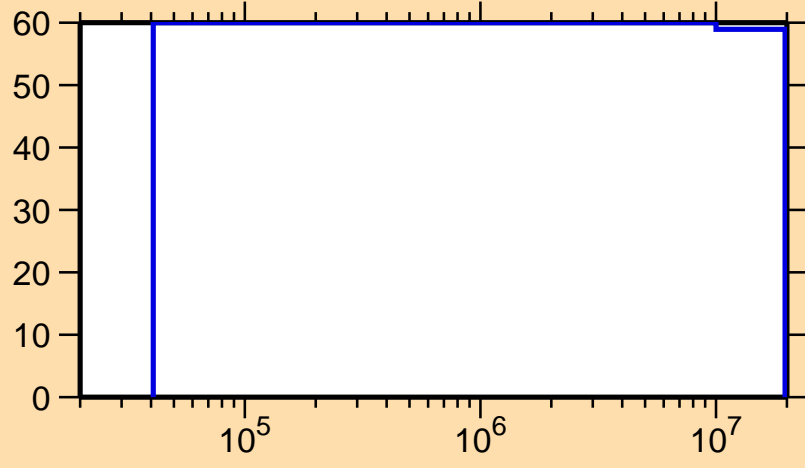
\Delta\sigma/\sigma vs. E for ^{110}\text{In}(n,n_1)
