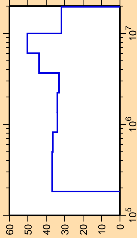
\Delta\sigma/\sigma vs. E for ^{110}\text{In}(n,n_2)
