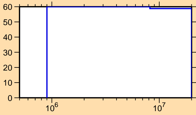
\Delta\sigma/\sigma vs. E for ^{110}\text{In}(n,n_1)
