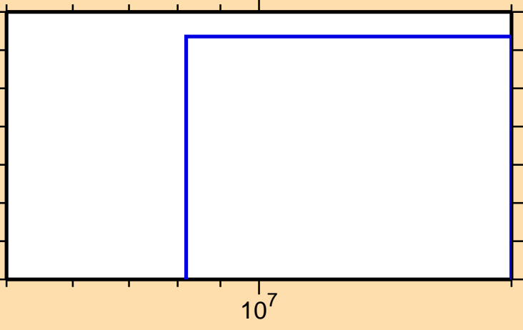
\sigma vs. E for ^{110}\text{In}(n,\text{pd})
