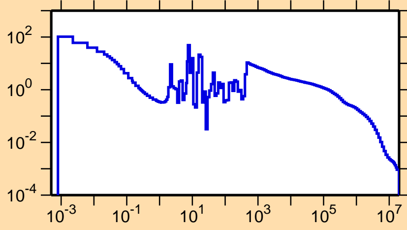
\sigma vs. E for ^{110}\text{In}(n,\gamma)
