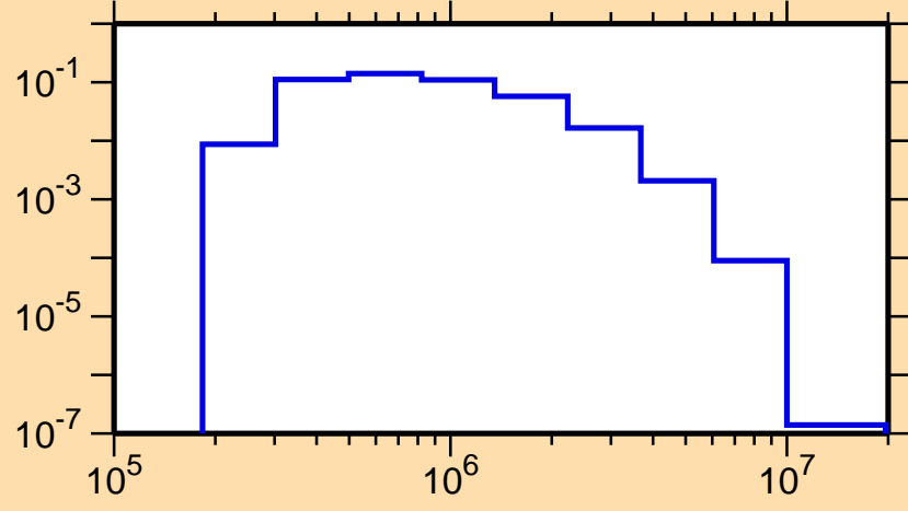
\sigma vs. E for ^{110}\text{In}(n,n_3)
