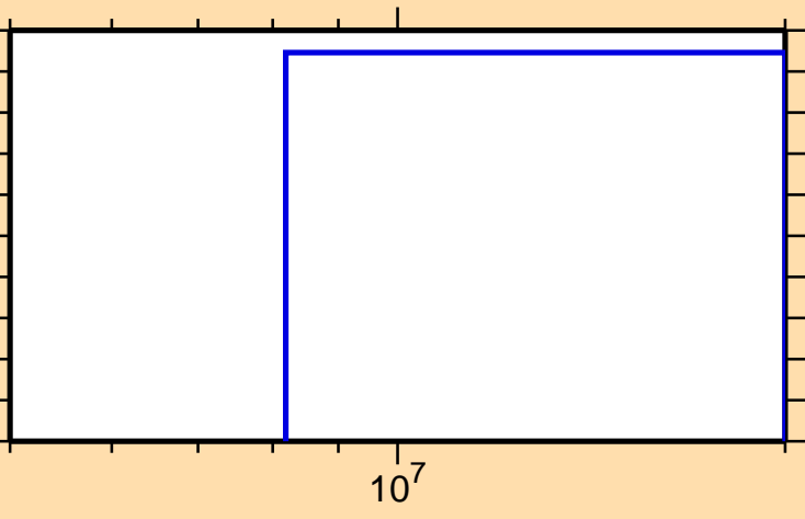
\sigma vs. E for ^{110}\text{In}(n,2np)
