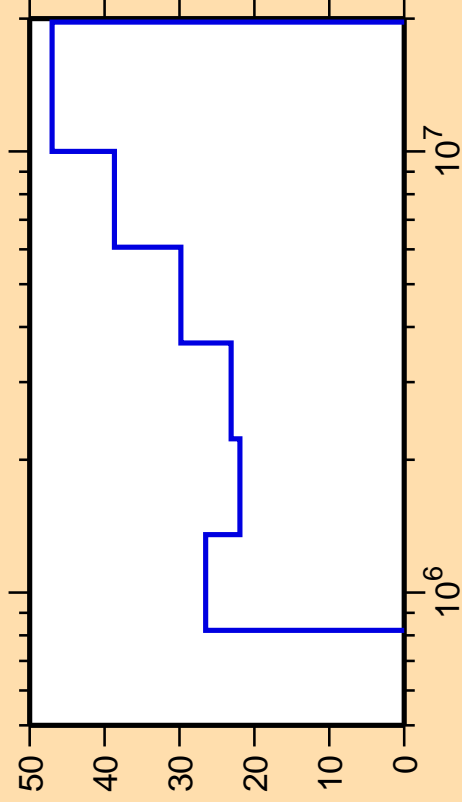
\Delta\sigma/\sigma vs. E for ^{111}\text{In}(n,n_4)
