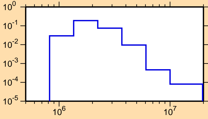
\sigma vs. E for ^{111}\text{In}(n,n_4)
