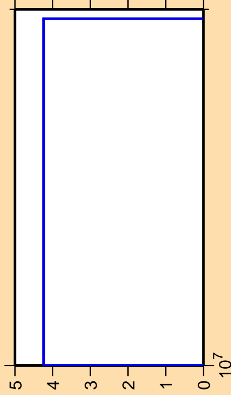
\Delta\sigma/\sigma vs. E for ^{111}\text{In}(\text{mt117})
