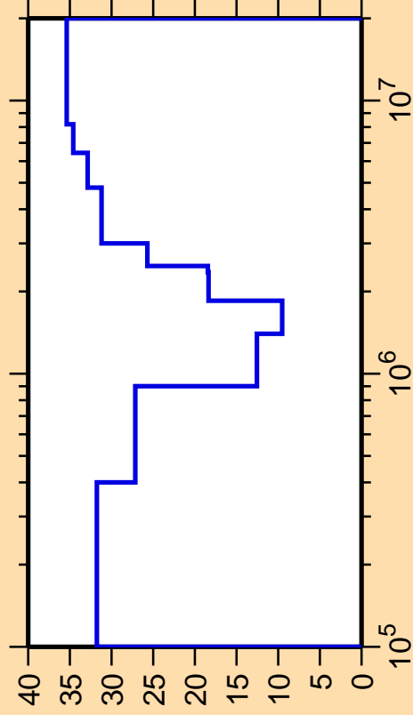
\Delta\sigma/\sigma vs. E for ^{111}\text{In}(n,n_2)
