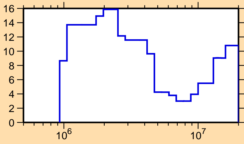
\Delta\sigma/\sigma vs. E for ^{112}\text{In}(n,\text{tot.})
