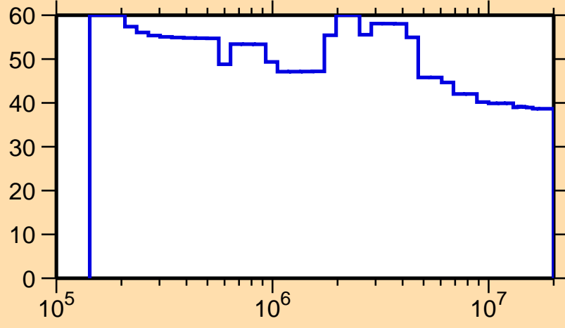
\Delta\sigma/\sigma vs. E for ^{112}\text{In}(n,n_1)
