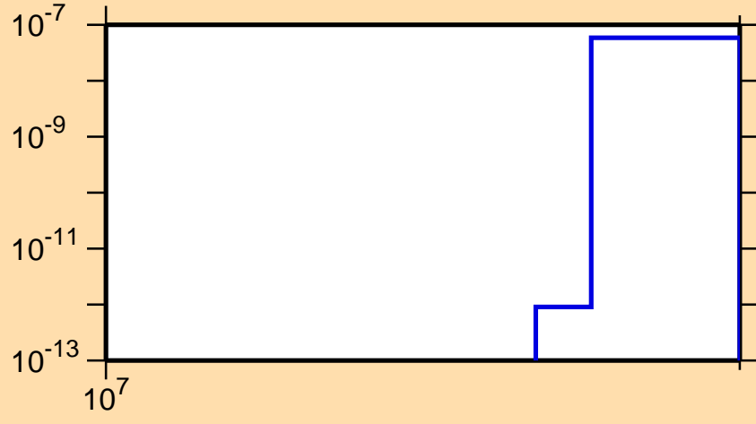
\sigma vs. E for ^{112}\text{In}(n,nt)
