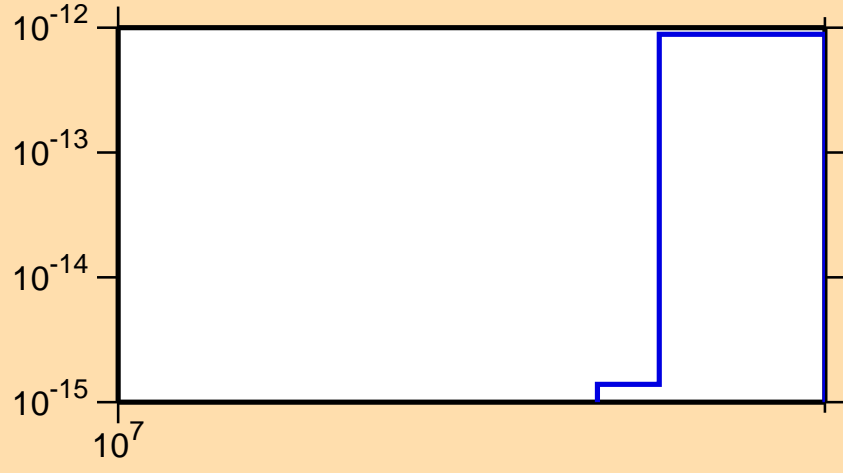
\sigma vs. E for ^{112}\text{In} (mt 45)
