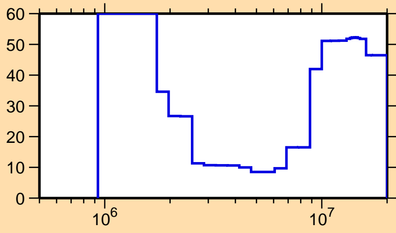
\Delta\sigma/\sigma vs. E for ^{112}\text{In}(n,n\text{cont.})
