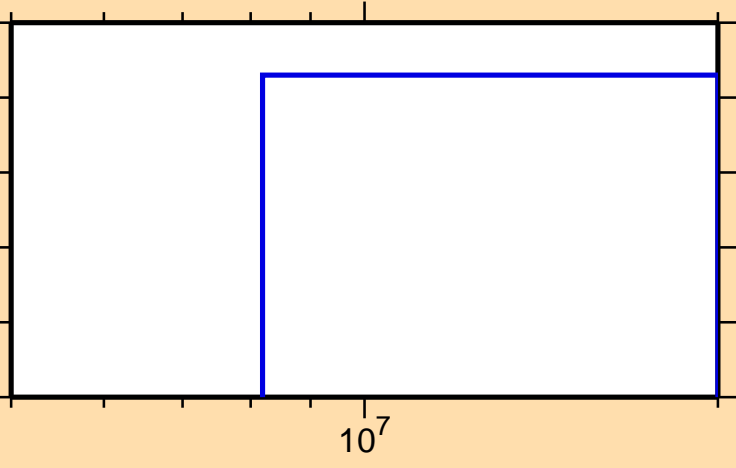
\sigma vs. E for ^{112}\text{In}(n,\text{He3})
