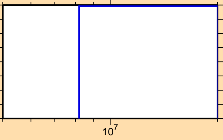
\sigma vs. E for ^{112}\text{In}(n,p\alpha)
