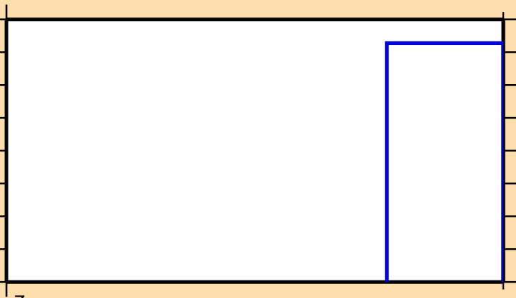
\sigma vs. E for ^{112}\text{In}(n,3n)
