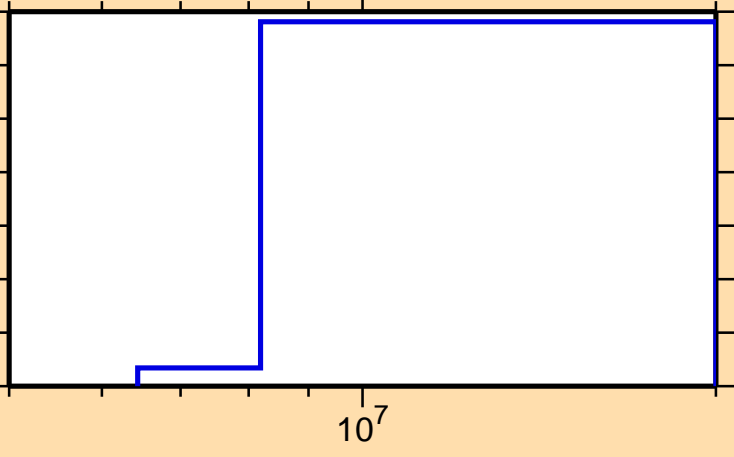
\sigma vs. E for ^{112}\text{In}(n,n\alpha)
