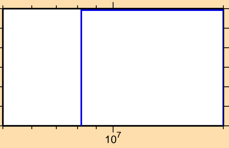
\sigma vs. E for ^{112}\text{In}(n,3n)
