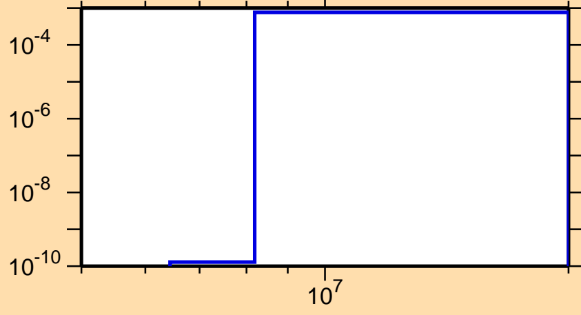
\sigma vs. E for ^{113}\text{In}(n,\alpha)
