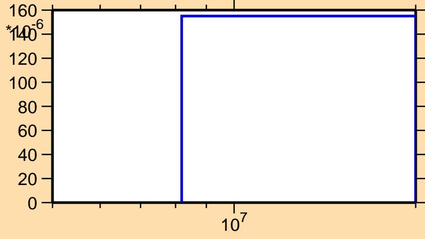
\sigma vs. E for ^{113}\text{In}(n,t)
