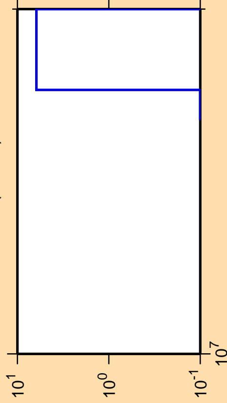
\Delta\sigma/\sigma vs. E for ^{113}\text{In} (mt 45)
