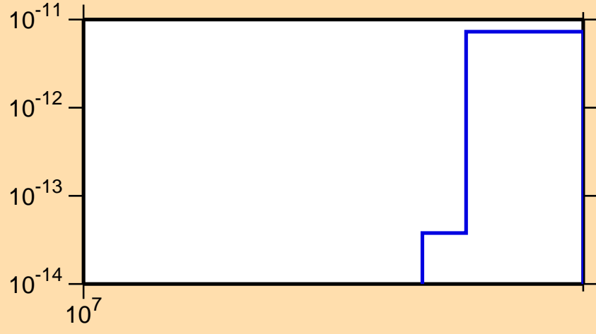
\sigma vs. E for ^{113}\text{In} (mt 45)
