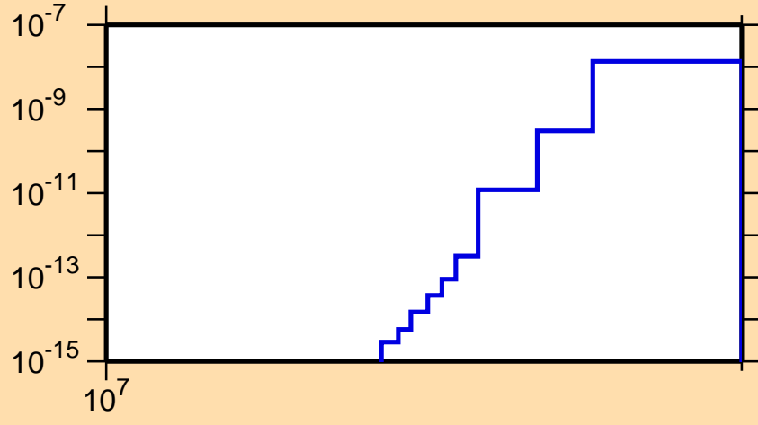
\sigma vs. E for ^{113}\text{In}(n,\text{He}3)
