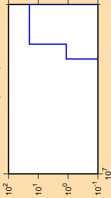
\Delta\sigma/\sigma vs. E for ^{113}\text{In}(\text{mt117})
