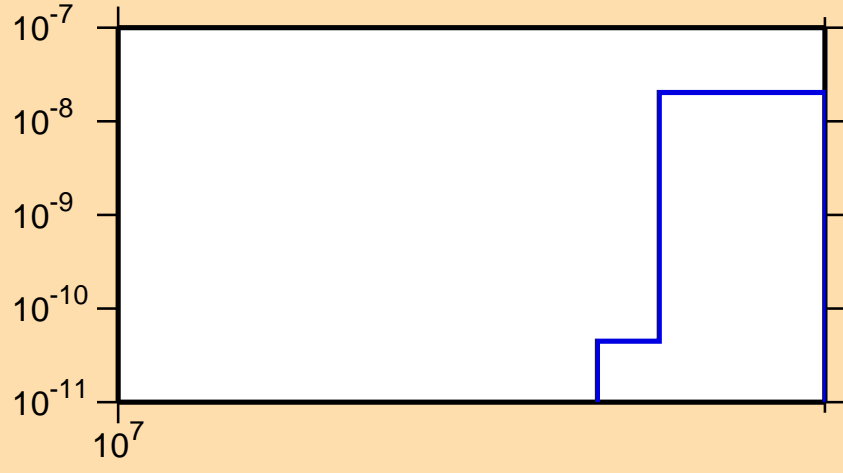
\sigma vs. E for ^{113}\text{In}(n,2n\alpha)
