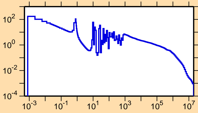
\sigma vs. E for ^{114}\text{In}(n,\gamma)
