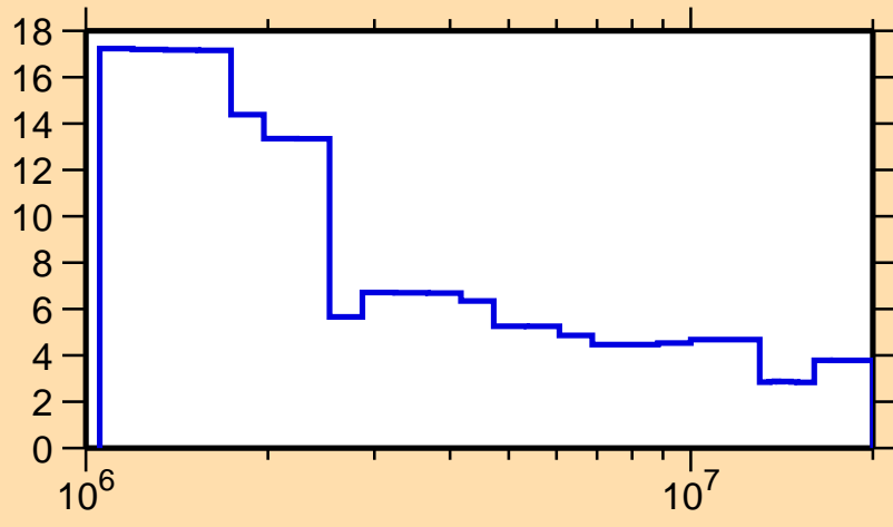
\Delta\sigma/\sigma vs. E for ^{114}\text{In}(n, n_{\text{nonel}})
