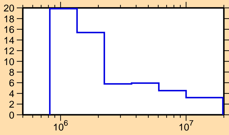
\Delta\sigma/\sigma vs. E for ^{114}\text{In}(n,n\text{onel.})
