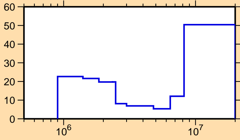
\Delta\sigma/\sigma vs. E for ^{114}\text{In}(n,n\text{cont.})
