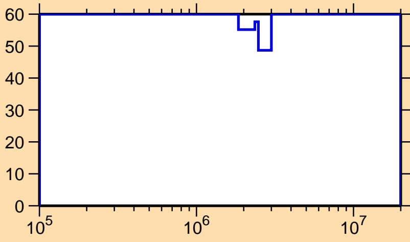
\Delta\sigma/\sigma vs. E for ^{114}\text{In}(n,n_1)
