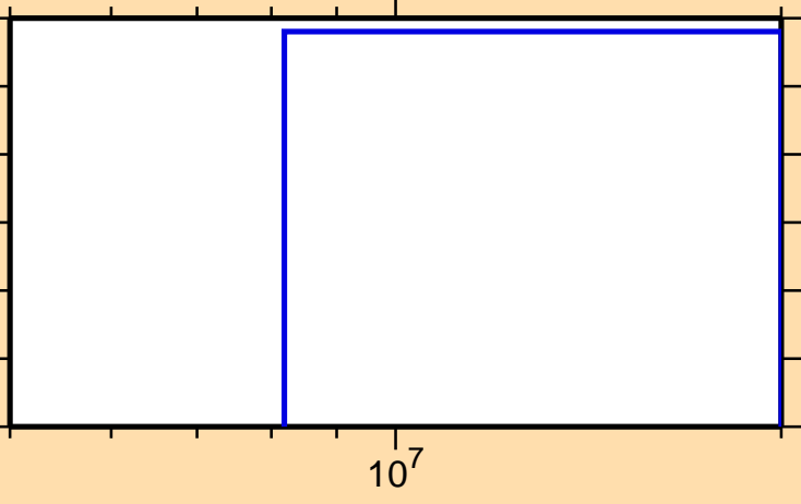
\sigma vs. E for ^{114}\text{In}(n,\text{He3})
