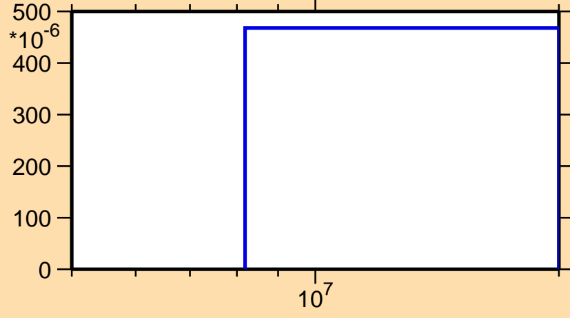
\sigma vs. E for ^{115}\text{In}(n,3n)
