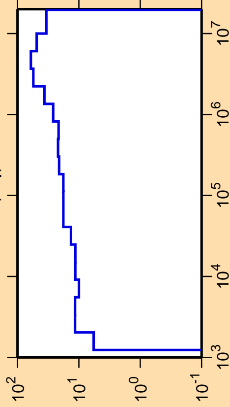
\Delta\sigma/\sigma vs. E for ^{116}\text{In}(n,\gamma)
