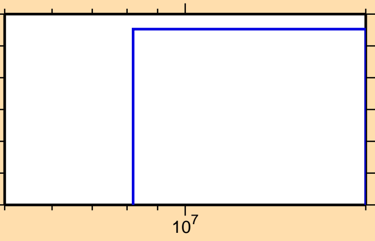
\sigma vs. E for ^{116}\text{In}(n,2n\alpha)
