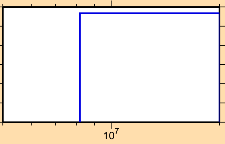
\sigma vs. E for ^{117}\text{In}(n,np)
