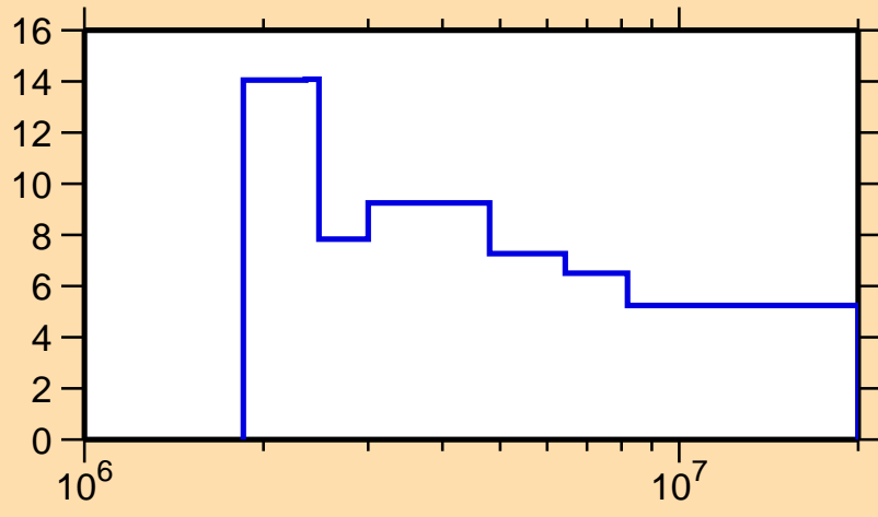
\Delta\sigma/\sigma vs. E for ^{117}\text{In}(n, n_{\text{nonel}})
