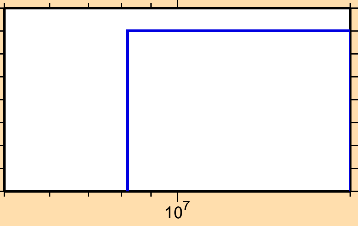
\sigma vs. E for ^{117}\text{In}(n,\alpha)
