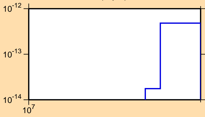
\sigma vs. E for ^{117}\text{In}(n,p\alpha)
