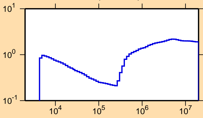
\sigma vs. E for ^{117}\text{In}(n,\text{nonel.})
