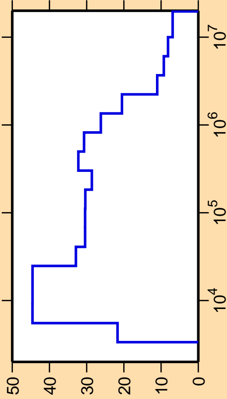
\Delta\sigma/\sigma vs. E for ^{117}\text{In}(n,\text{nonel.})
