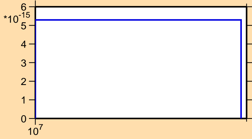
\sigma vs. E for ^{117}\text{In}(n,p\alpha)
