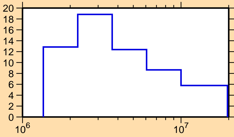
\Delta\sigma/\sigma vs. E for ^{117}\text{In}(n, el.)
