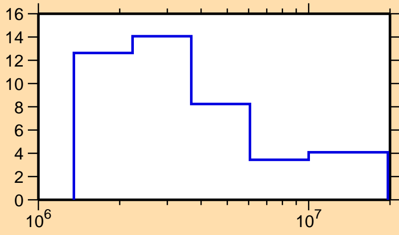
\Delta\sigma/\sigma vs. E for ^{117}\text{In}(n,\text{tot.})
