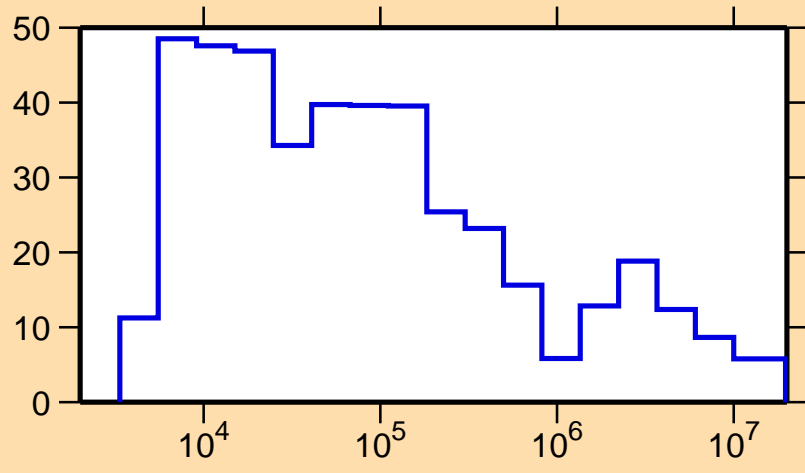
\Delta\sigma/\sigma vs. E for ^{117}\text{In}(n,\text{el.})
