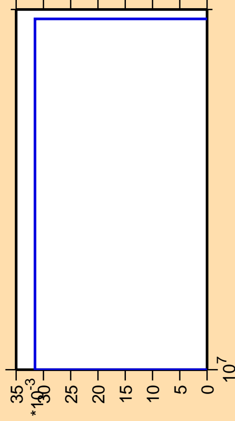
\Delta\sigma/\sigma vs. E for ^{117}\text{In}(n,p\alpha)
