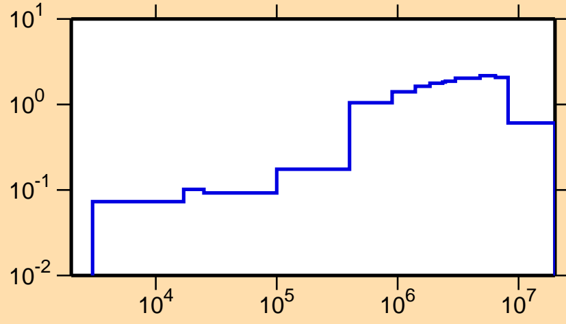
\sigma vs. E for ^{117}\text{In}(n,\text{inel.})
