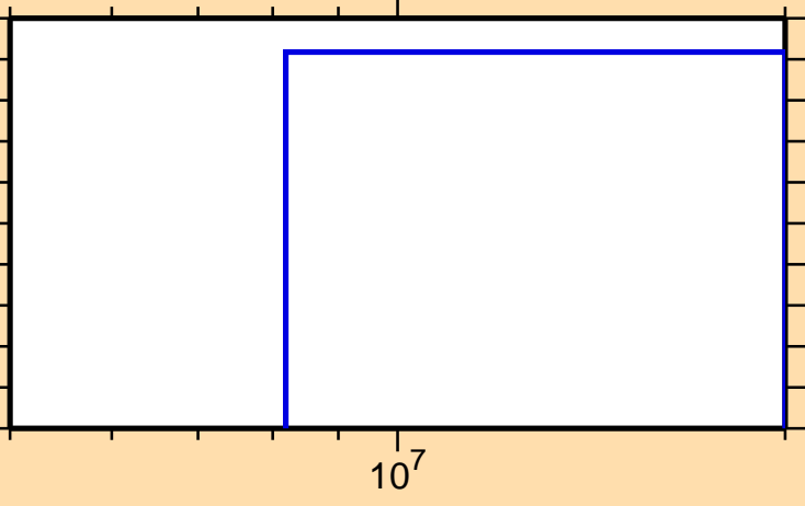
\sigma vs. E for ^{117}\text{In}(n,t)
