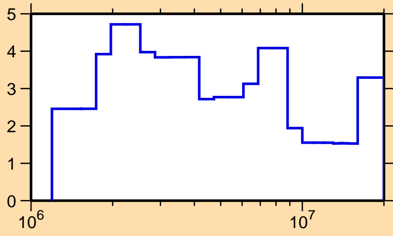
\Delta\sigma/\sigma vs. E for ^{118}\text{In}(n, el.)
