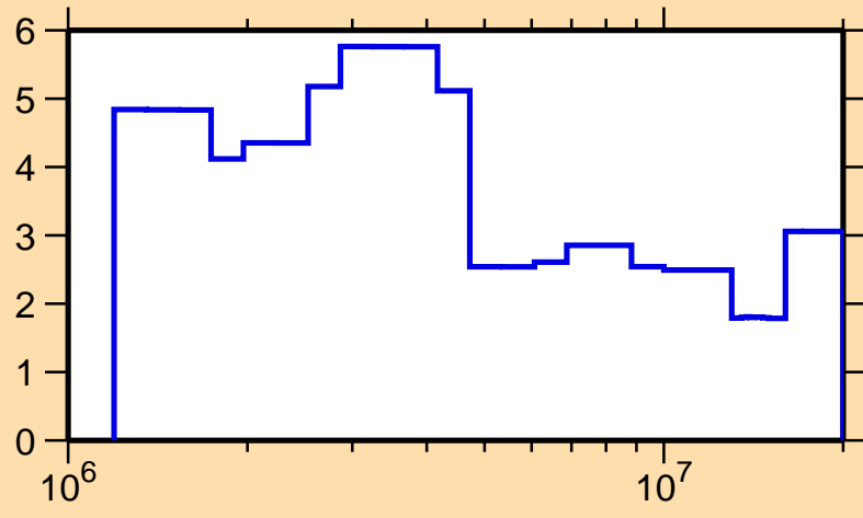
\Delta\sigma/\sigma vs. E for ^{118}\text{In}(n, n_{\text{nonel}})
