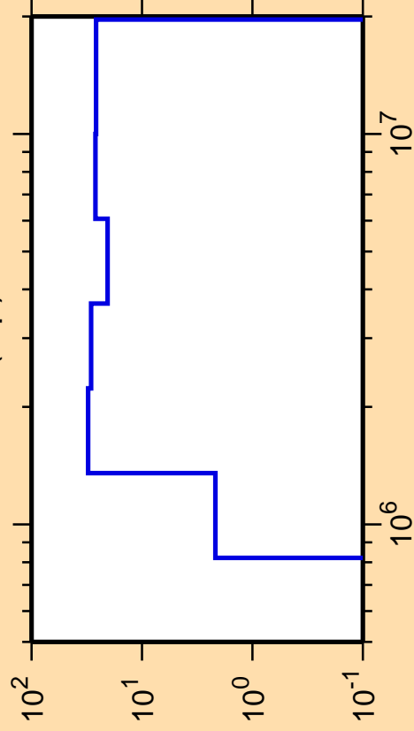
\Delta\sigma/\sigma vs. E for ^{118}\text{In}(n,p)
