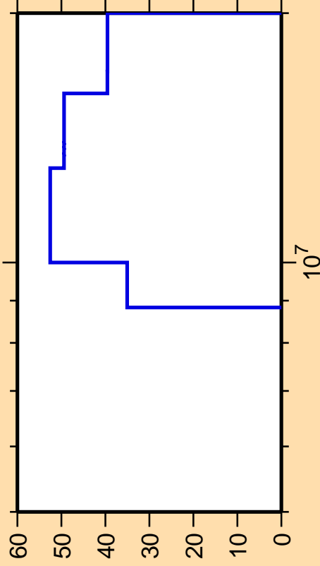
\Delta\sigma/\sigma vs. E for ^{118}\text{In}(n,np)
