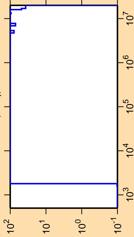
\Delta\sigma/\sigma vs. E for ^{118}\text{In}(n,n_1)
