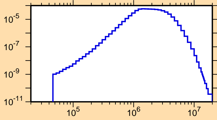
\sigma vs. E for ^{118}\text{In}(n,n_1)
