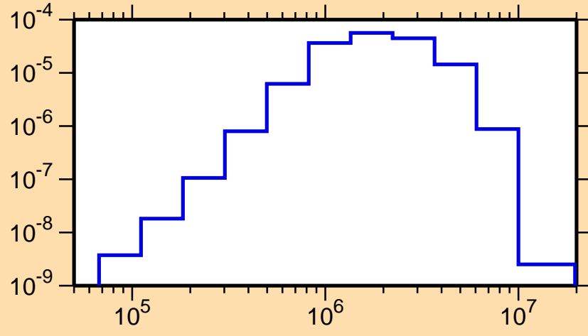
\sigma vs. E for ^{118}\text{In}(n,n_1)
