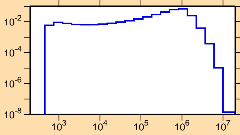
\sigma vs. E for ^{118}\text{In}(n,n_2)
