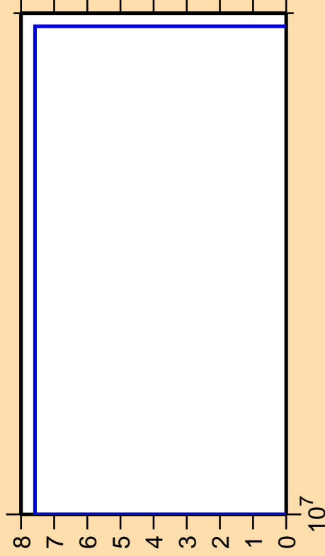
\Delta\sigma/\sigma vs. E for ^{119}\text{In}(n,2np)
